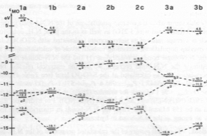
Fig. 2. Orbital-correlation diagram for the 3 highest HOMO's and the lowest LUMO in the seven N_3H_3 -isomers 1-3 at the 6-31G** level
