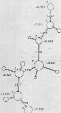
Figure 1. MNDO optimized structure of the model 2-oxoethyl-2-oxoethylidene-phosphorane; calculated atomic charges and bond lengths.
