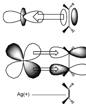
Figure 1. Silver(I)–alkene bonding: \pi – s^* donation (top) and d – \pi^* back-donation (middle) interactions as relevant for the \text{Ag}^+-(\text{C}_2\text{H}_4)_n complexes under study ( n = 1-4, 6 ).
