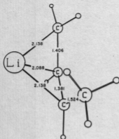
Fig. 2. The 3-21G geometry of cis -crotyllithium. Note the orientation of the \text{CH}_3 group and the bending of \text{C}(2)\text{-H} towards lithium.
